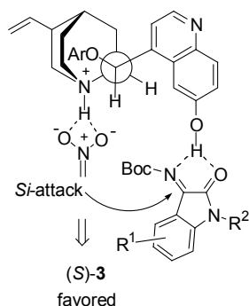
Figure 3 Stereochemical model
