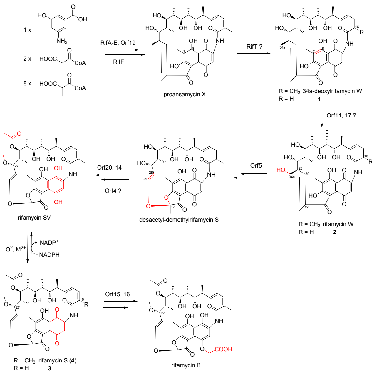
Scheme 1 Biosynthetic pathway of rifamycins
