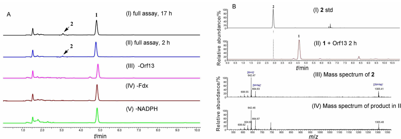
Figure 2 Functional verification of rif-orf13 through in vitro enzymatic assays
