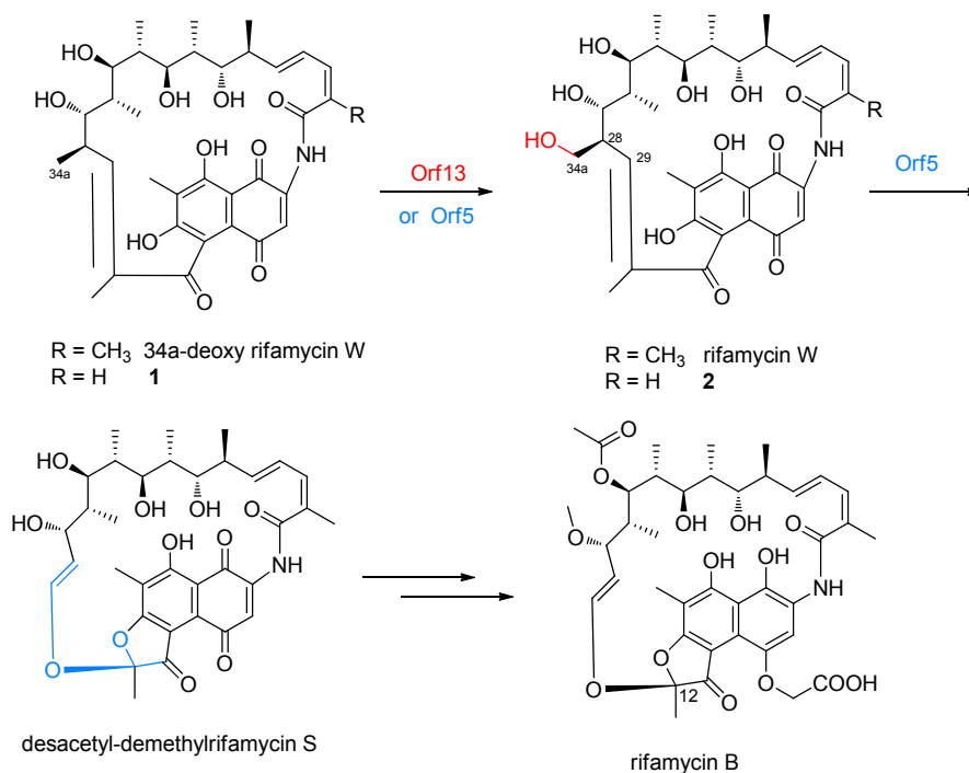
Scheme 2 Proposed function of Orf13 in the biosynthesis of rifamycins
