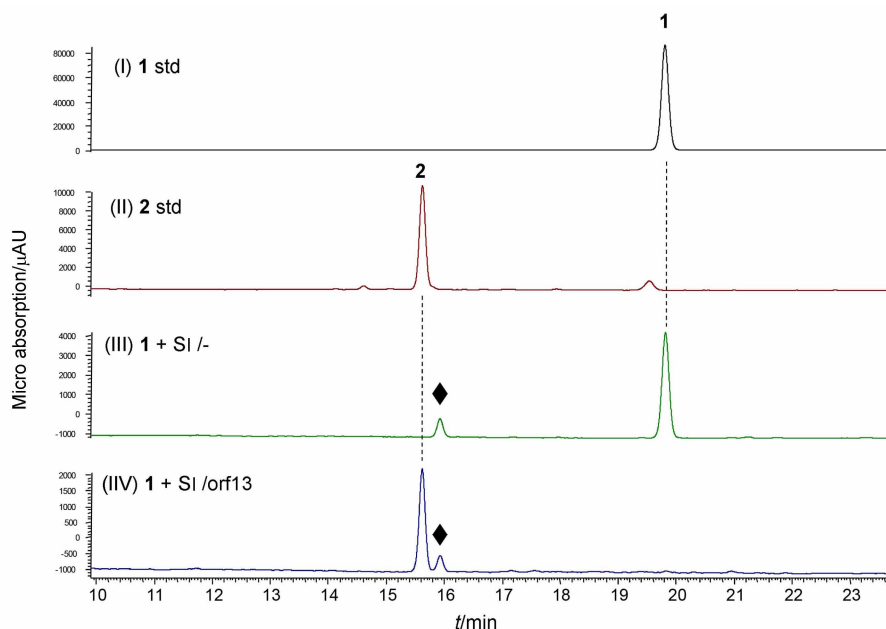
Figure 1 Heterologous expression and feeding experiments of rif-orf13
